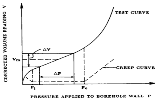
Figure 3: Pressure change - Volume change curve
